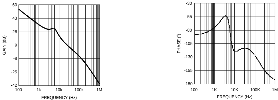
Figure 55. Overall Loop Gain and Phase
