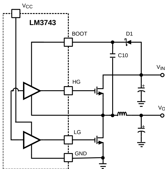
Figure 48. Charge Pump Circuit and Driver Circuitry
